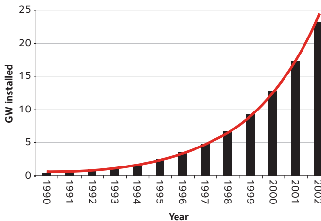
Figure 2.1 European Union cumulative installed wind power capacity 6,7
