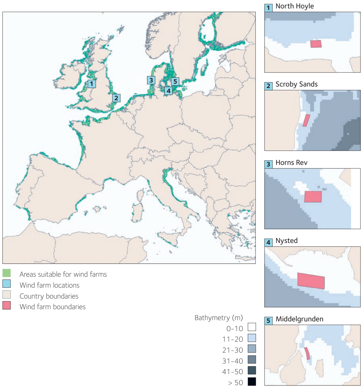
Figure 3.2 Commercial-scale offshore wind farms existing or under construction
