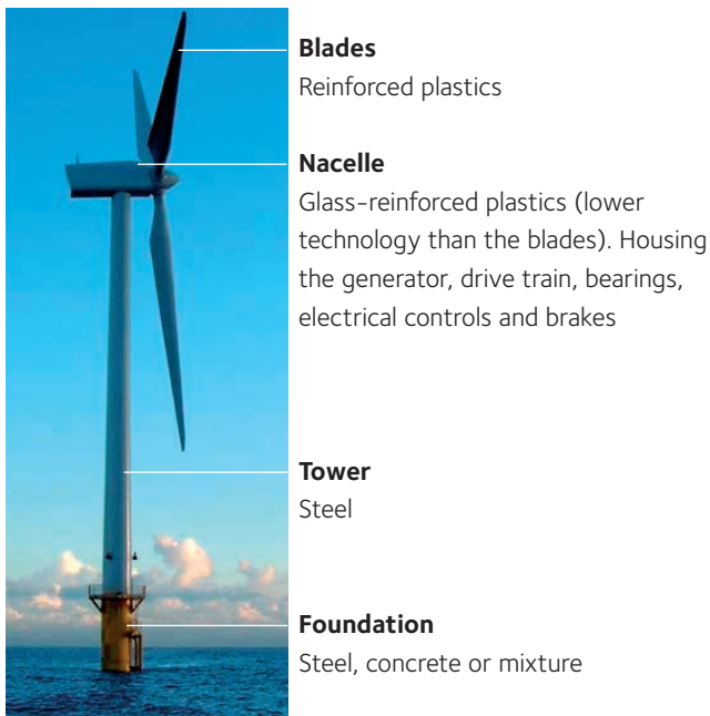
Figure 5.1 The main components of a wind turbine
